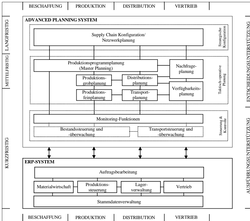
Abb. 6 Supply Chain Planning Matrix
