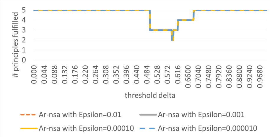
Figure 43: Non-detailed threshold evaluation using Ar-nsa . The term principles fulfilled refers to the principles not disproven in the experimental evaluation.
