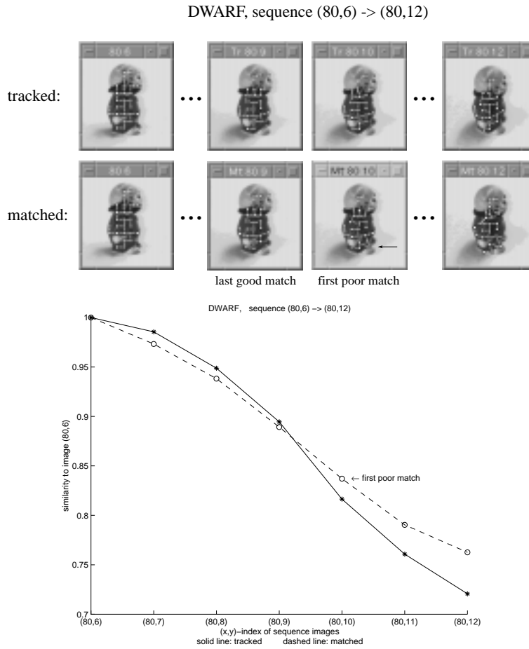
Figure 6: Correspondences for Object “Dwarf”.
