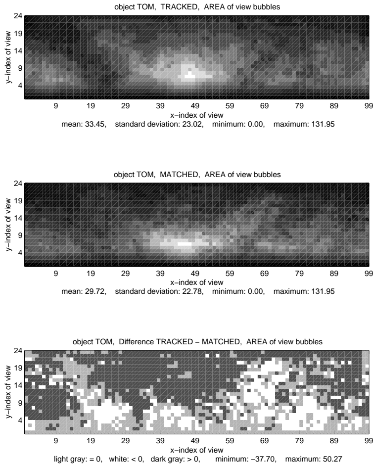
Figure 3: Distribution of View Similarities for Object “Tom”.
